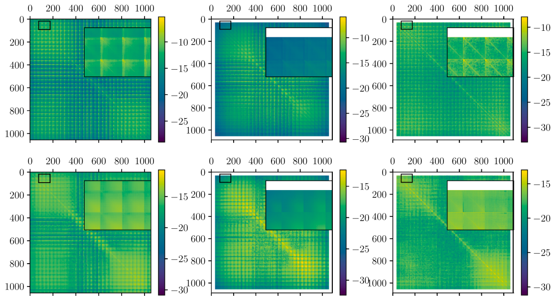
Fig. B.1. Logarithm of the absolute value of the covariance between the magnitudes of the Fourier coefficients. A total of 33 Fourier coefficients are computed along horizontal cross-sections of the domain, giving rise to the squared pattern. The figure displays the covariance for the horizontal velocity (left), vertical velocity (middle), and temperature (right), computed for the reference data (top row) and the measured sub-grid force (bottom row).
